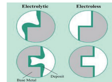
Electrolytic vs Electroless Nickel
